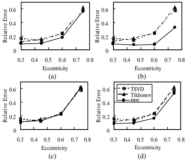
Fig. 2 Eccentricity vs. relative errors. The scalp potentials were contaminated with (a) GWN and (b) edge-, (c) center-, and (d) on side-concentrated non-uniform noise.
