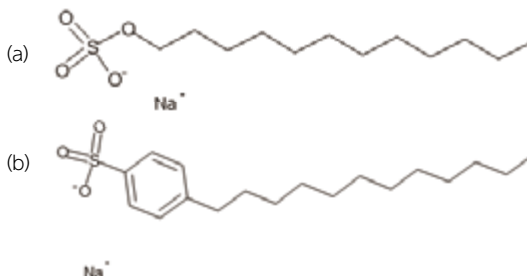
Fig. 1 (a) Sodium Dodecyl Sulfate (b) Sodium Dodecylbenzene Sulfonate
